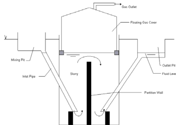
Figure 2: Floating cover digester
