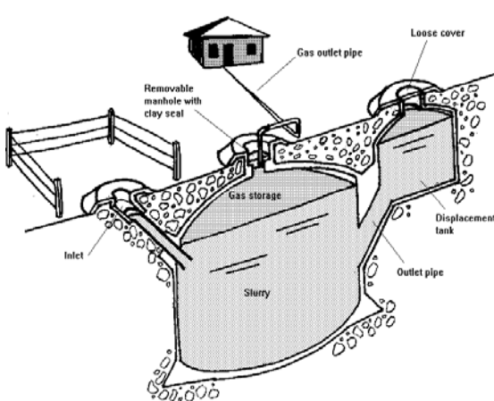
Figure 1: Fixed dome digester
